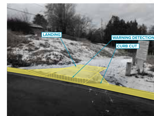
G-2 CONSTRUCT ACCESSIBLE ENTRANCE AT BONNEVILLE DRIVE
