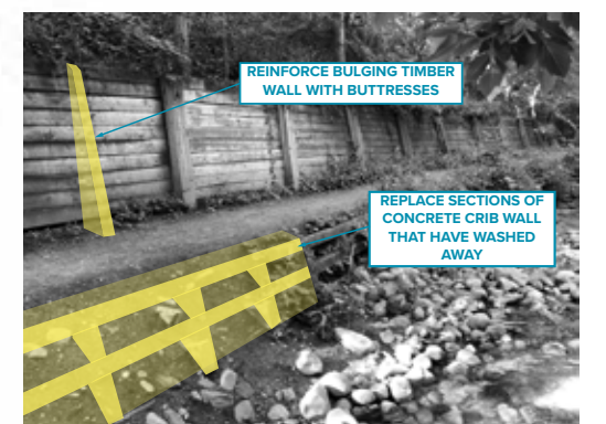
F-2 TIMBER AND CRIB WALL REPAIRS
