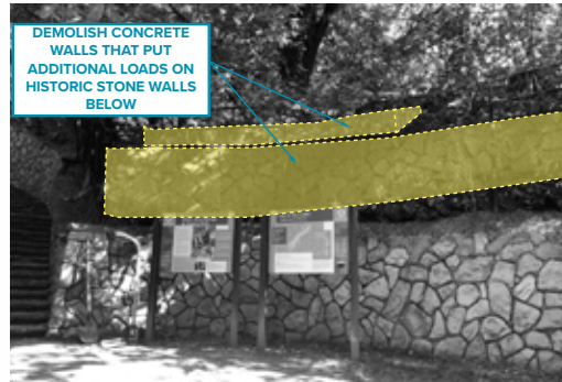
E-1 REMOVE STACKED CONCRETE WALL
